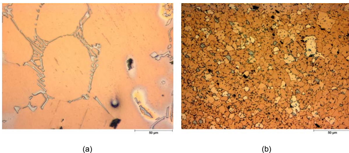
Figure 5.17: Microstructural changes in the consumable in dissimilar MRI230D/AZ91D-T6 welds. In (a) the typical \text{Mg}(\text{Al},\text{Ca}) eutectics along the grain boundaries and in (b) the same material after welding at mid-thickness at the rotational centre (see position “G” Figure 4.22).
