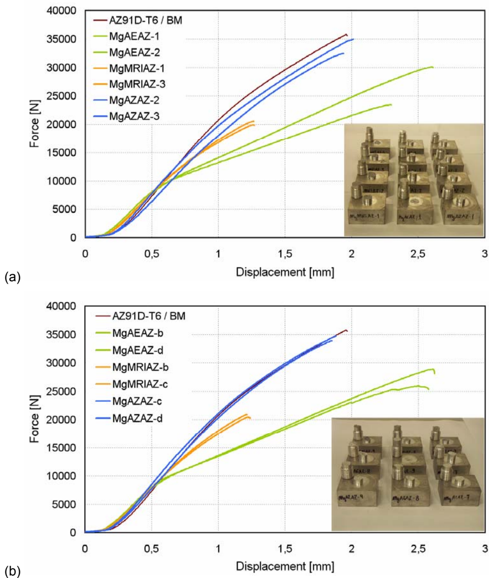
Figure 4.28: Pull-out test results for \varnothing 8 mm/10 mm upsetting welds.
