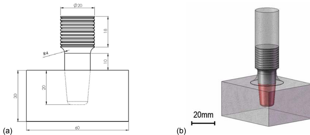
Figure 3.9: Pull-out specimen geometry (a) and position of the sample in relation to the joint (b).
