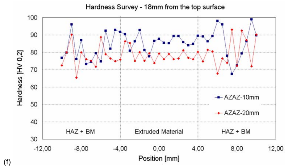
Figure 4.27: Horizontal hardness profiles along the joints at 2 mm and 18 mm from the top surface.
