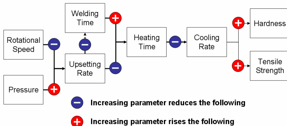
Figure 2.13: Parameter influence in Friction Welding.
