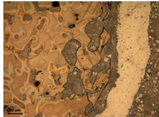
Figure 2.22: Macrograph of a dissimilar FHPP weld using an aluminium AA6082 stud and a magnesium AZ91D-T6 base plate [126] .
