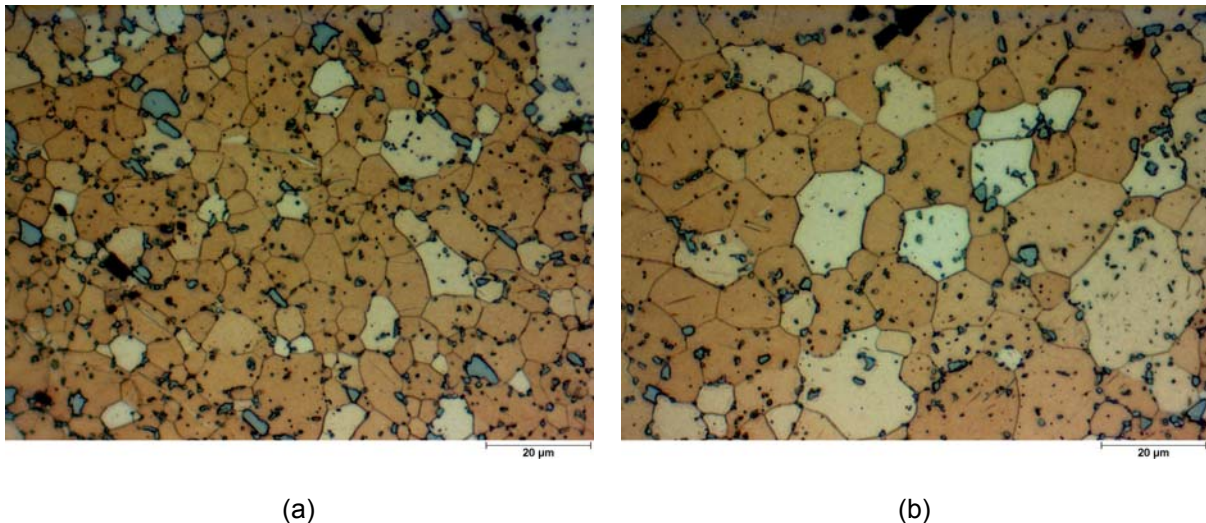
Figure 5.18: Grain size assessment within the extruded material. In (a) the microstructure in the “f” (average diameter: 7.3 \mu\text{m} ) and (b) in the “h” (average diameter: 11.8 \mu\text{m} ) position.
