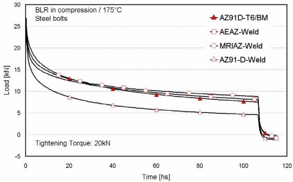
Figure 4.35: Typical bolt load compressive stress retention curves at 175 °C for AZ91D-T6 similar and AEAZ, MRIAZ dissimilar welds covering the entire test. Base material behaviour is also presented for comparison.
