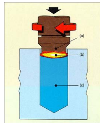
Figure 2.16: FHPP principle.
