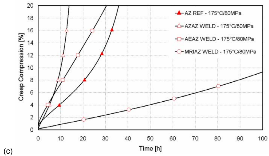
Figure 5.28: In (a), (b) and (c), the compression creep curves are plotted for similar and dissimilar welded samples at 125 °C, 150 °C and 175 °C respectively. Curves AZAZ REF were also plotted at different temperatures and represent the AZ-BM behaviour for further comparison.
