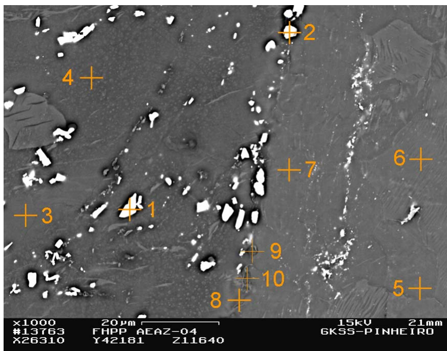
Figure 4.21: Weld interface of the dissimilar AE42/AZ91D-T6 FHPP welded joint. Backscattered electron micrograph showing points for EDS analysis in particles distributed along the joint line.
