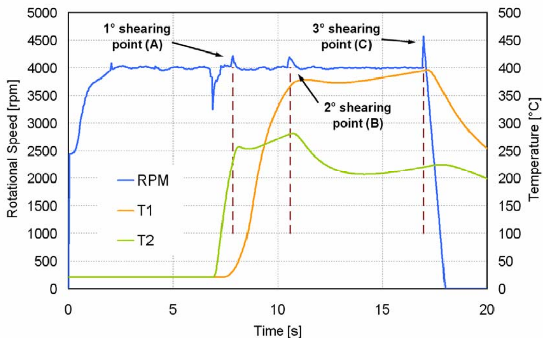
Figure 5.7: Welding parameter measurements of weld AZAZ-3C. The shearing phenomena observed on the macrograph could be clearly identified.
