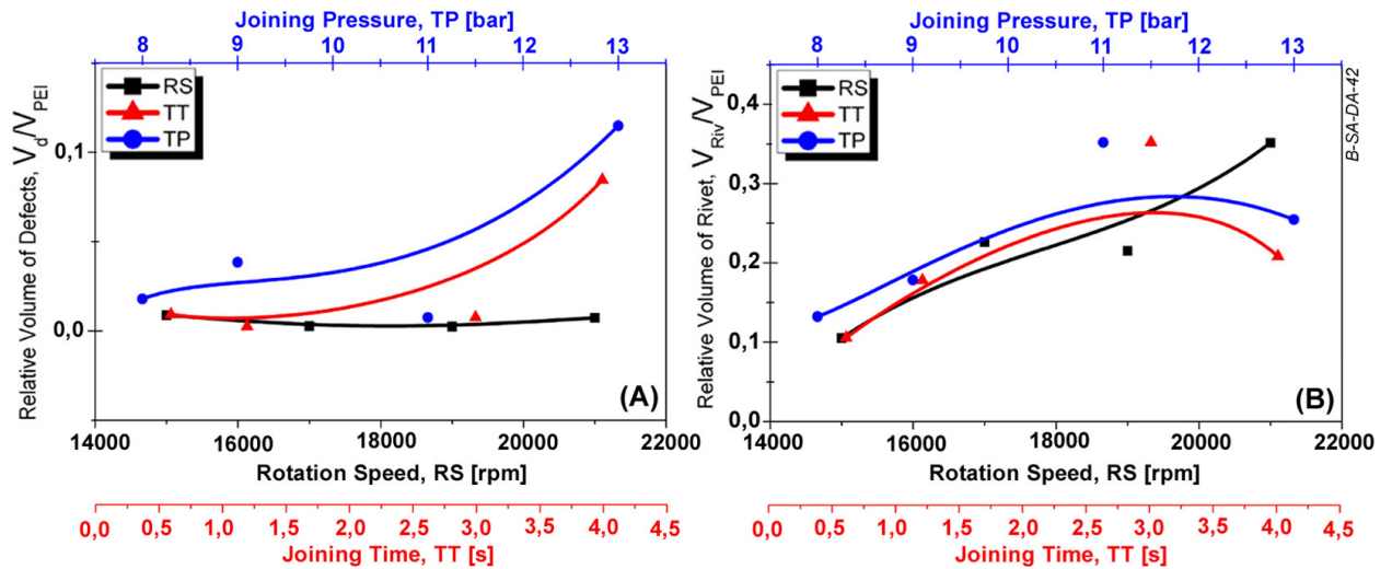
Figure 39. A) Relative volume of defects (flaws), V_d/V_{PEI} for RS, TT and TP comparison study. B) Relative volume of rivet inside the polymeric base plate, V_{Riv}/V_{PEI} , for RS, TT and TP comparison study.
