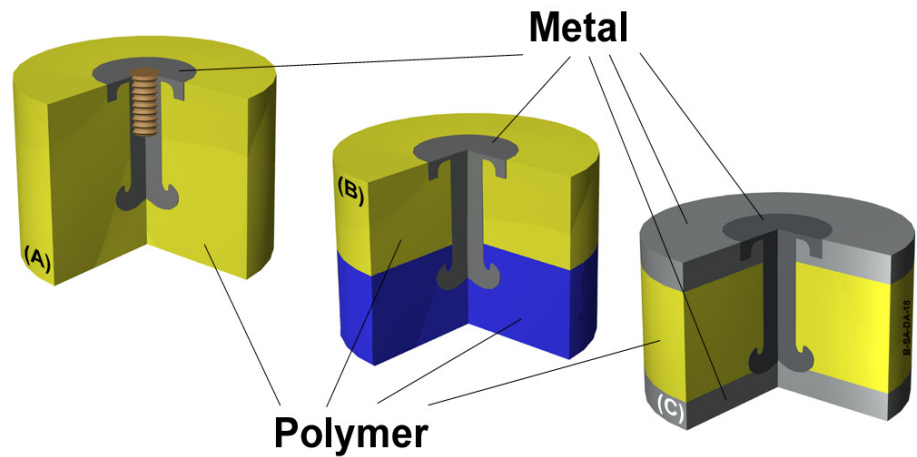
Figure 22. Possible configurations of hermetic sealed friction riveted joints. A) point-on-plate insert-joint. B) overlap joint. C) sandwich type joint
