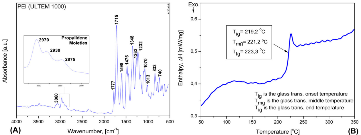
Figure 20. A) Experimental infrared spectrum of PEI (ULTEM 1000) base material with major peaks marked. B) experimental DSC-thermogram showing T_g -range.
