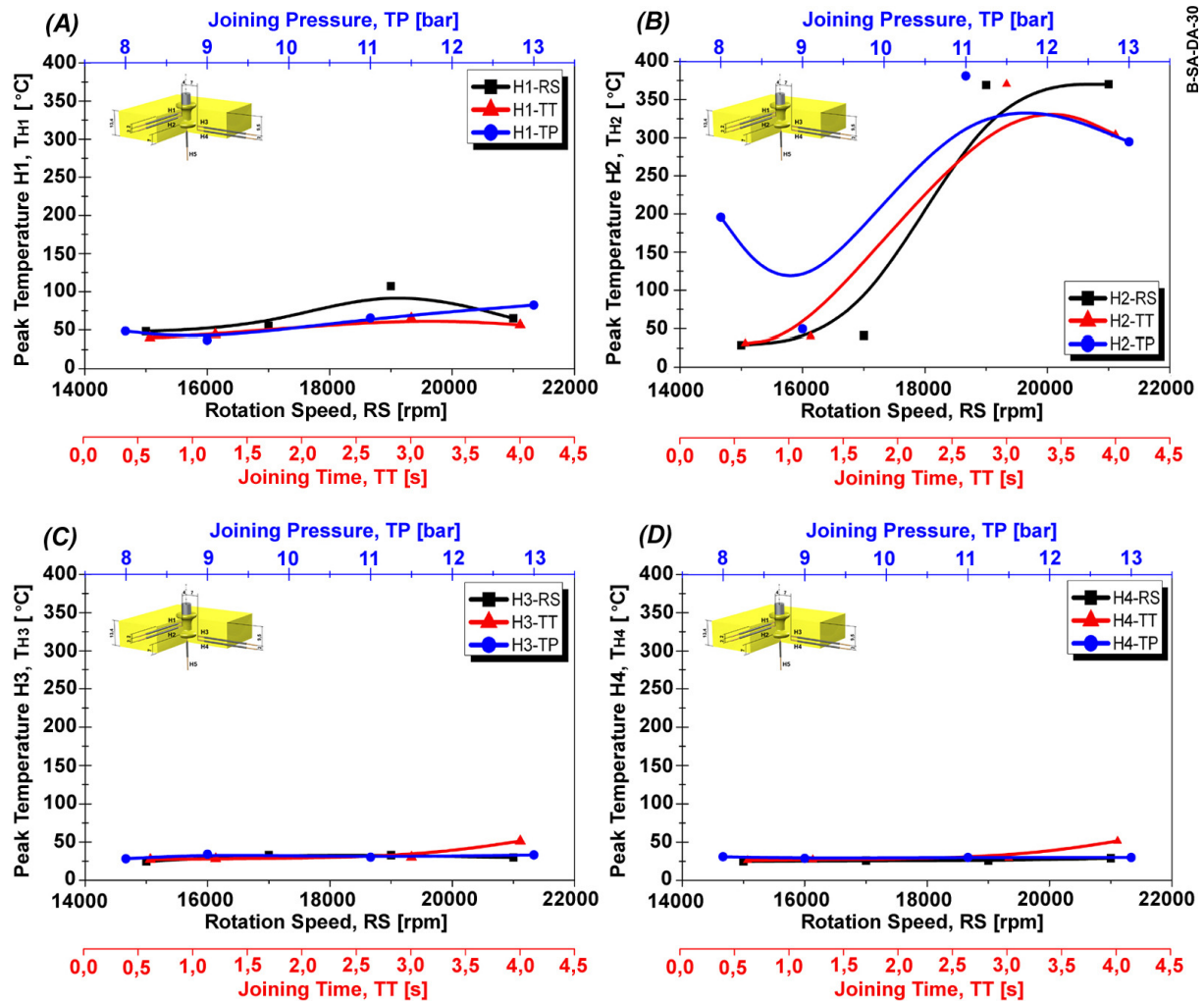
Figure 31. Thermometric results for PEI/AA2024-T351 point-on-plate comparison joints. A) Peak temperatures of H1-thermocouples (depth= 2 mm; distance to joint centre= 4 mm). B) Peak temperatures of H2-thermocouples (depth= 4 mm; distance to joint centre= 4 mm). C) Peak temperatures of H3-thermocouples (depth= 9,5 mm; distance to joint centre= 7 mm). D) Peak temperatures of H4-thermocouples (depth= 11,5 mm; distance to joint centre= 7 mm).
