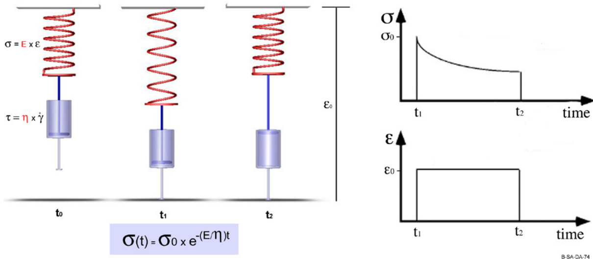
Figure 64. Maxwell Model for viscoelastic stress relaxation in plastics. Symbols: \sigma , is the stress \eta , the viscosity, \tau the shear stress, \gamma the shear rate, \epsilon the strain and t the time.
