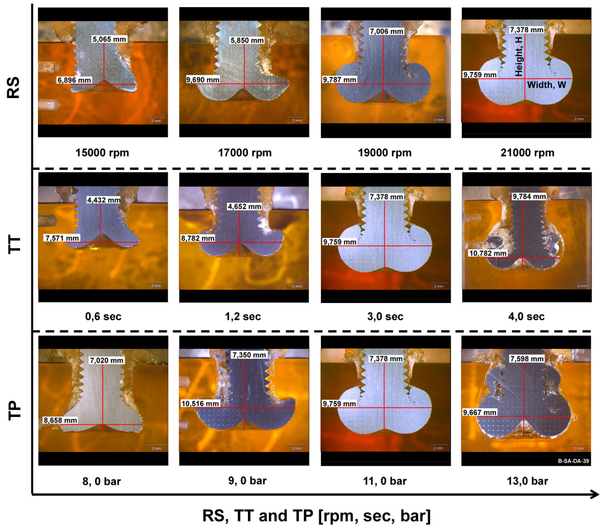
Figure 40. Non-etched LOM-macrographs of cross sections taken from the middle of the joint. h -values are related to vertical lines and w -values to horizontal lines, 25X. Horizontal cylindrical holes near to rivet's shaft in samples 15000 rpm, 0,6 sec, 4,0 sec, 8,0 bar and 9,0 bar are the holes for thermocouple temperature measurements.
