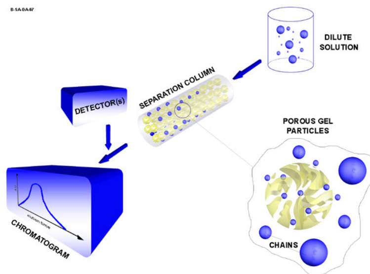
Figure 15. Schematic view of a GPC-system.
