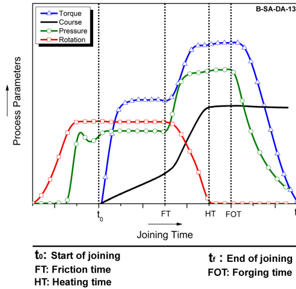
Figure 8. Scheme of a friction riveting joining diagram.
