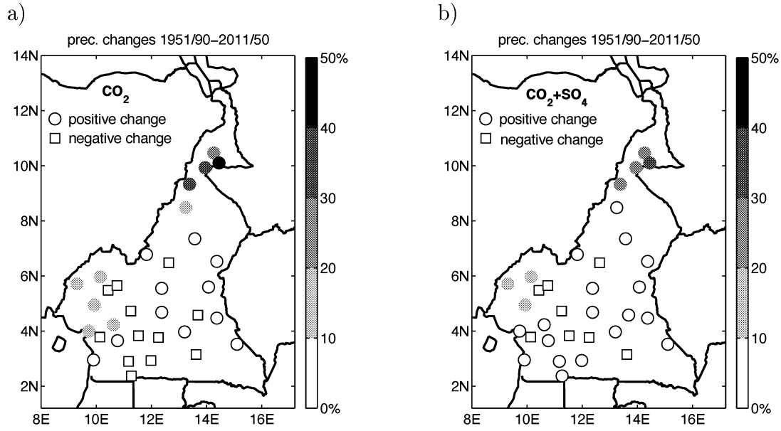
Figure 7: Downscaled local rainfall changes derived from a GCM experiment under IPCC IS92a scenario: a) CO 2 only; b) CO 2 + SO 4 . Changes are expressed in percentage relative to the observed period 1951-1990.
