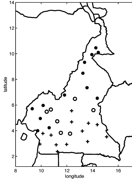
Figure 3: Clusters found by SOFM based on standardised anomalies for the period 1951-1990. C1 (*), C2 (○) and C3 (+).
