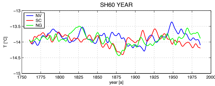
Figure 5.6: High latitude Southern hemispheric temperatures south of 60° S for the different experiments. Note the decrease of temperatures within the second half of the 20th century. The time series have been smoothed with a 10-years Gaussian low pass filter.
