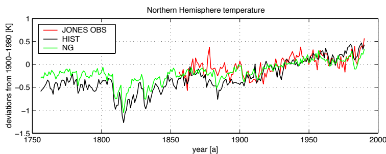
Figure 5.14: Northern hemispheric temperature deviations [ ^{\circ}\text{C} ] from the period 1900-1980 for the Jones et al. (1999b) observational data and the HIST and NG experiments. Note the coincidence of the curves during the 20th century but with a temperature trend within the HIST experiment which is too strong.
