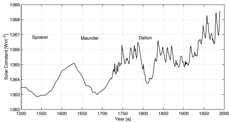
Figure 2.2: Evolution of the solar 'constant' since 1500. The most prominent anomalous periods are the Spörer, the Maunder and the Dalton Minima (after Crowley 2000).
